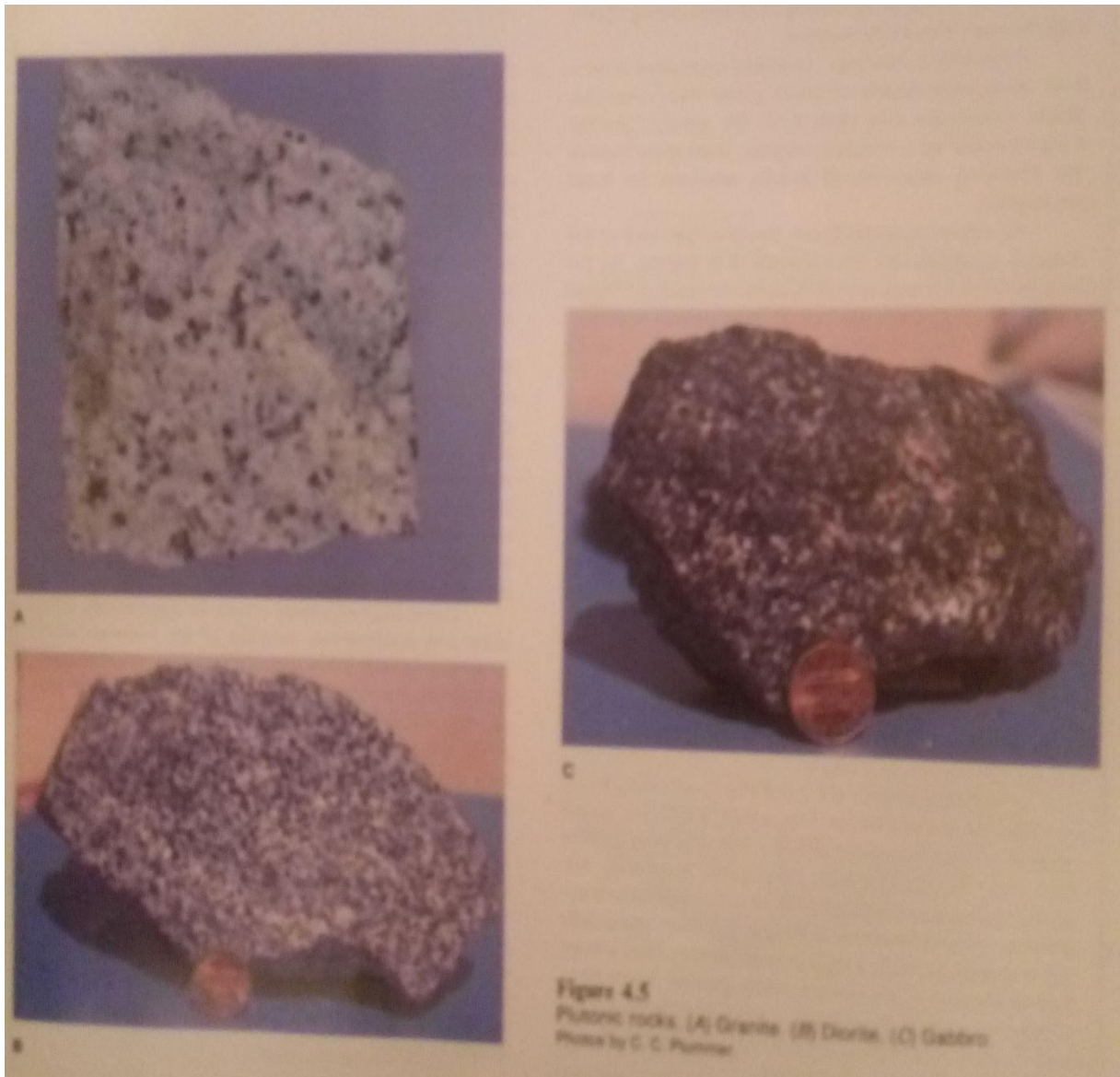
Figure 3 roches plutoniques (a) granite, (b) diorite, (c) gabbro.
